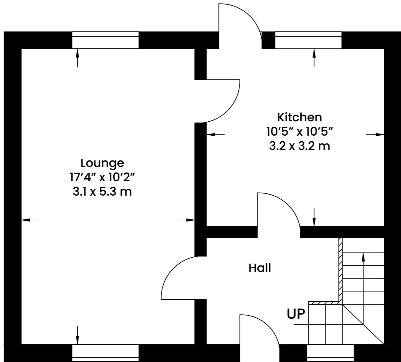
Ground Floor
