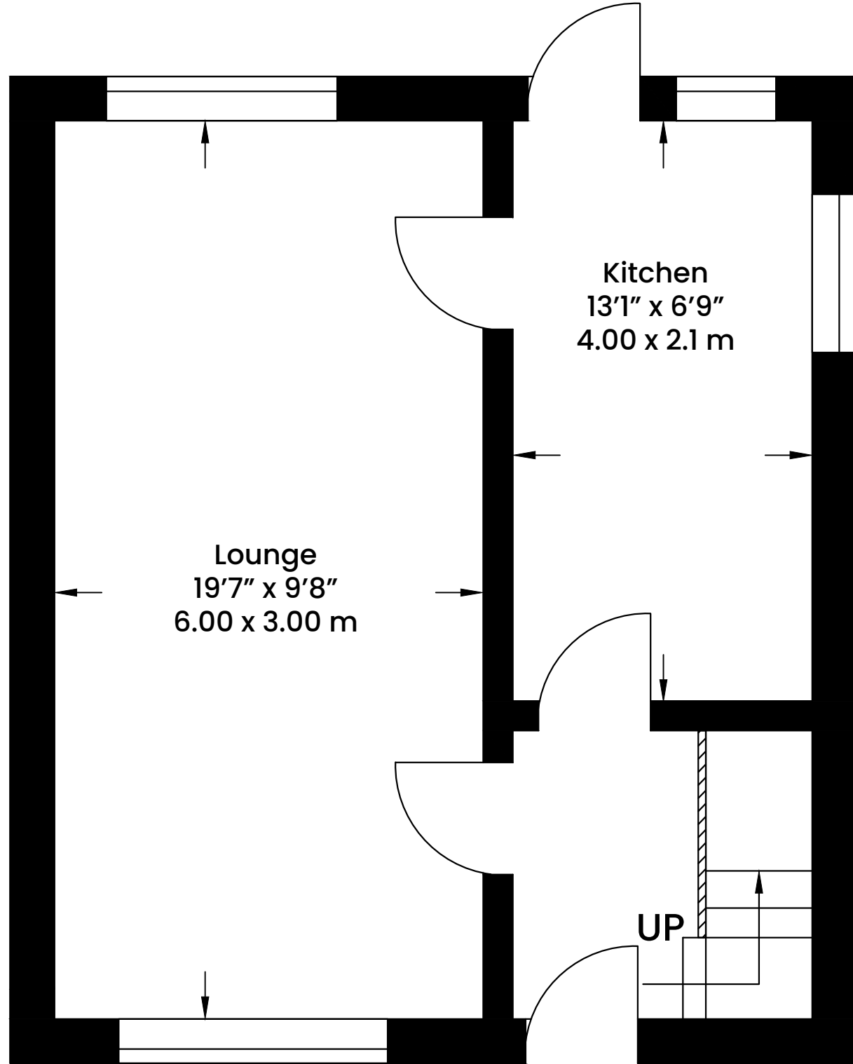
Ground Floor
